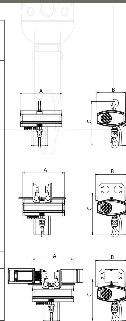
Inverter HoistMaster4
